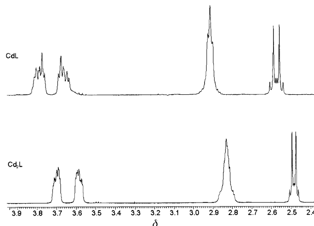
Fig. 6 Comparison of the ^1\text{H} NMR spectra of \text{CdL} and \text{Cd}_2\text{L} with \text{L} = \mathbf{1} at pH 7 ( [\text{CdL}] = 5 \times 10^{-3} \text{ mol dm}^{-3} , [\text{Cd}_2\text{L}] = 5 \times 10^{-3} \text{ mol dm}^{-3} ).
